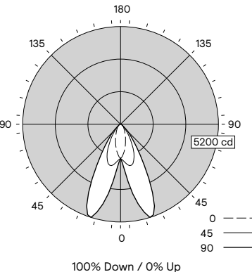
Performance 63° Symmetric Stack Beam MesoOptics louver Spacing Criteria: 0.54/1.37
