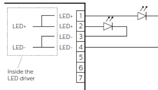
Schematic representation of iSet driver connections
