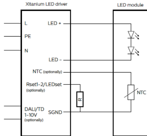
Schematic representation of Rset/LEDset driver connections
