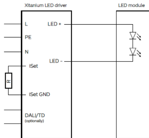
Schematic representation of iSet driver connections
