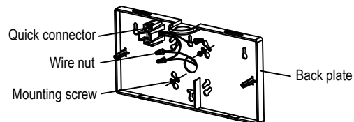
Wall mount-Top Power Feed
