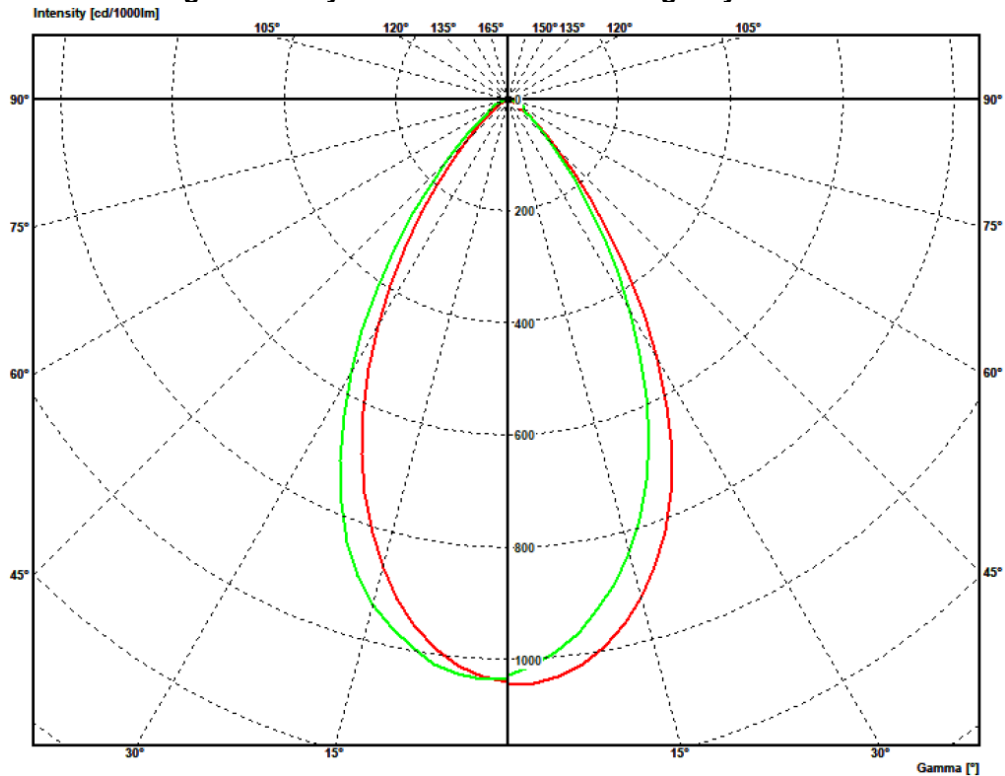
Light intensity distribution curves Emergency mode
