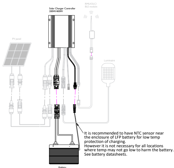
2a: Connection diagram for 200W-400W OCU
