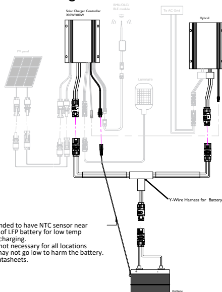
2d: Connection diagram for 600W HCU
