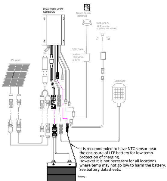
2e: Connection diagram for 300W OCU (Gen5)
