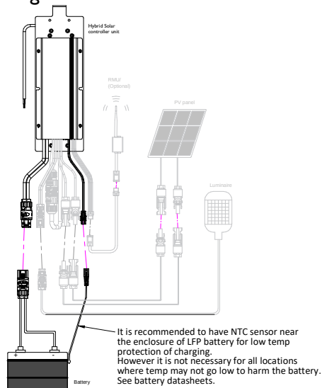
2f: Connection diagram for 300W HCU (Gen5)
