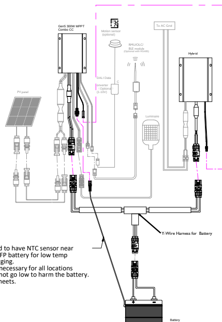
2f: Connection diagram for 300W HCU (Gen5)
