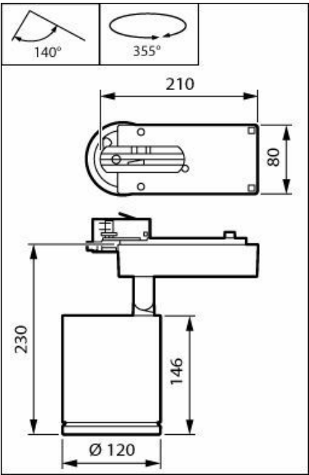
StyliD Evo Performance - Power supply unit - Beam angle 36° - 36° -
