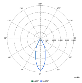
Polar Normal (separate) - ST333TI - 910505104617
