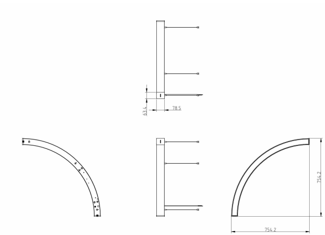
SP570P LED41/840 D150W6 90 SD CRV PSD
