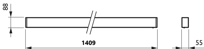
TrueLine NOC - 940 neutral white - Power supply unit with DALI interface - Push-in connector 5-pole - Aluminum
