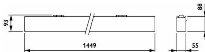
TrueLine OC - Tunable white - Power supply unit with DALI and SystemReady interface, InterAct ready - Push-in connector 3-pole - Aluminum
