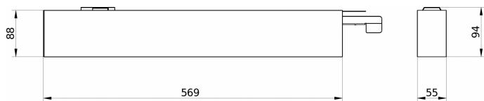
TrueLine OC - 940 neutral white - Power supply unit with DALI interface - Push-in connector 5-pole - Aluminum
