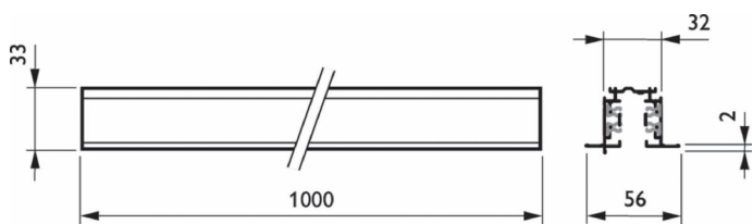
RBS750 5C6 L1000 BK (XTSCF6100-2)
