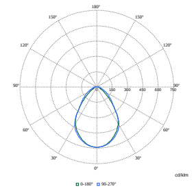
Polar Normal (separate) - RC450BI - 910505103956
