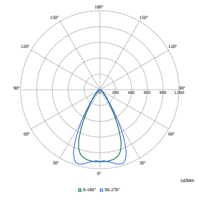
Polar Normal (separate) - RC450BI - 910505103963
