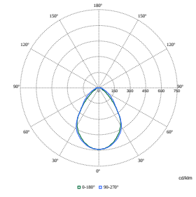
Polar Normal (separate) - RC450BI - 910505103982
