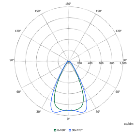
Polar Normal (separate) - RC450BI - 910505103961
