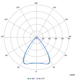
Polar Normal (separate) - RC450BI - 910505103973
