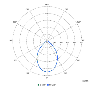
Polar Normal (separate) - RC450BI - 910505103945
