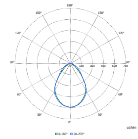
Polar Normal (separate) - RC450BI - 910505103952
