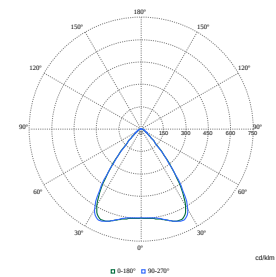
Polar Normal (separate) - RC450BI - 910505103977
