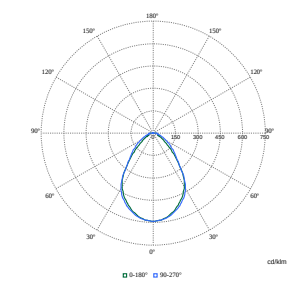
Polar Normal (separate) - RC450BI - 910505103953
