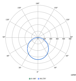
Polar Normal (separate) - RC340BI - 910925867012
