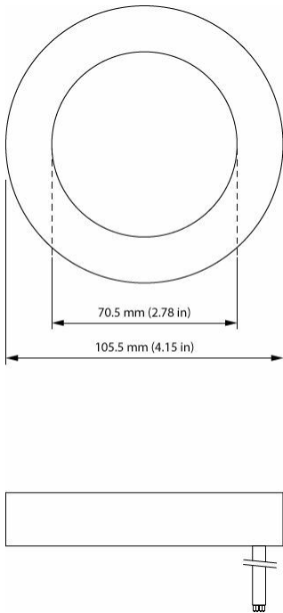
LCU7591 Amplight Leak Coil
