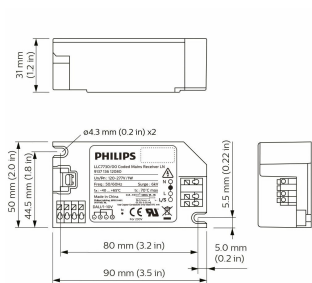
LLC7730/00 Coded Mains Receiver LN
