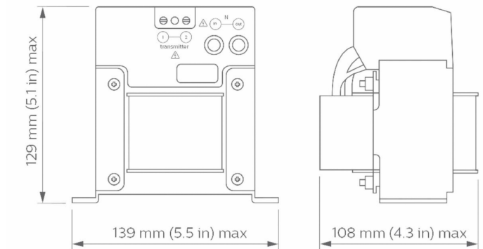
LCU7725/00 Coded Mains Transformer LN
