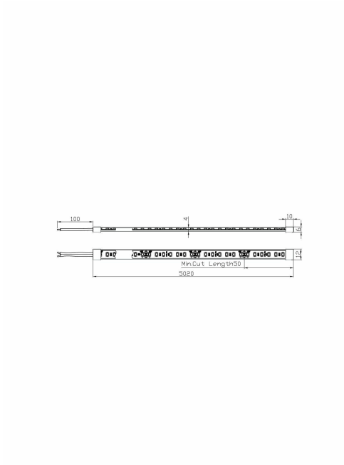
LS170S LED12 827 IP44 L5000 PRO
