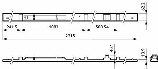
LL552X 160S/840 UE DIA NB WH
