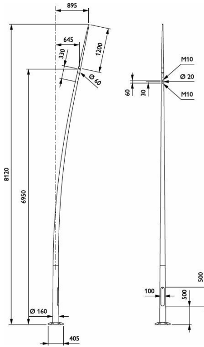
YHB709 CUR 7000 SPK 2xHOLE-M8-80 RAL
