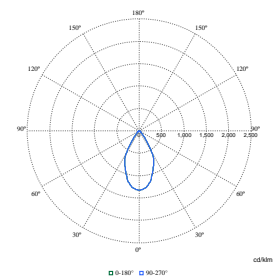
Polar Normal (separate) - GD601BI - 910505102202
