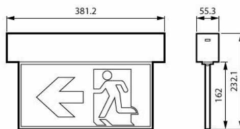
EM259C WL/CM EXIT SIGN M3 ELW WH
