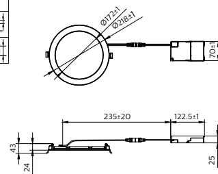
DN145B LED205/830_840 PSU WH
