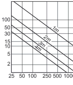
Accent Diagram - MC CDM-R Elite 70W/942 E27 PAR30L 30D
