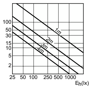
Accent Diagram - MASTER CDM-R111 Elite 70W/930 GX8.5 24D
