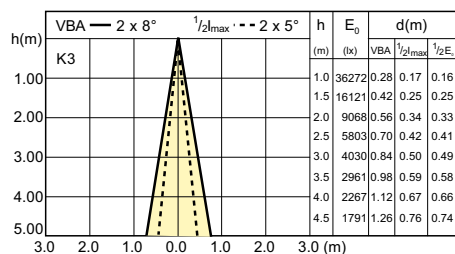
Beam diagram - MASTER CDM-R111 Elite 35W/930 GX8.5 10D
