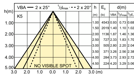
Beam diagram - MASTER CDM-R111 Elite 35W/930 GX8.5 40D
