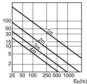
Accent Diagram - MASTER CDM-R111 Elite 35W/930 GX8.5 24D
