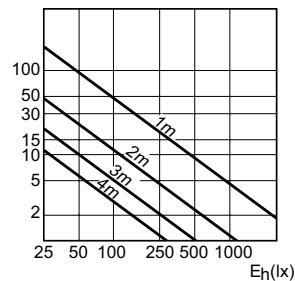
Accent Diagram - MASTER CDM-R111 Elite 35W/930 GX8.5 40D
