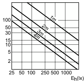
Accent Diagram - MASTER CDM-R111 Elite 35W/930 GX8.5 10D
