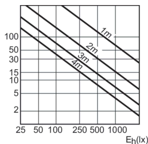
Accent Diagram - MASTER CDM-R111 Elite 70W/930 GX8.5 10D
