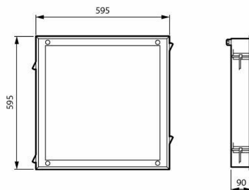
940 neutral white - Power supply unit with DALI interface - Push-in connector 5-pole
