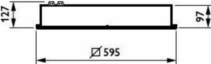
CR150B LED35S/840 PSD W60L60 IP54
