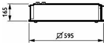
CR250B W60L60
