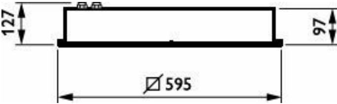
CR150B W60L60
