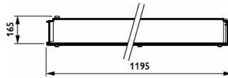
CR250B LED35S/840 PSU W30L120 IP65
