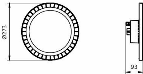
BY020P G3 LED105S/840 PSU WB GR
