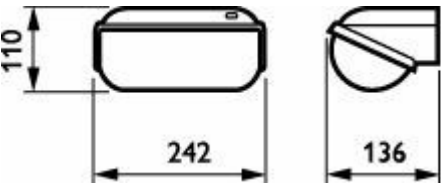
SECURITY LED 110 - LED Module 900 lm
