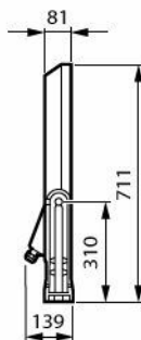
BVP657 LED930-4S/740 PSU A55-MB ALU
