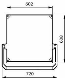
BVP657 LED930-4S/740 PSU A55-MB ALU
