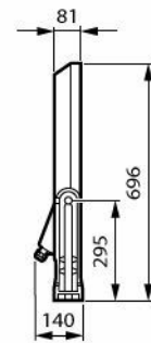
BVP656 LED600-4S/740 PSU DW10 ALU
