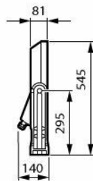
BVP655 LED300-4S/740 PSU DW10 ALU
