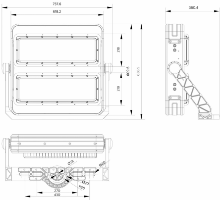
BVP582 LED1500/757 1200W A65NB R35BV
