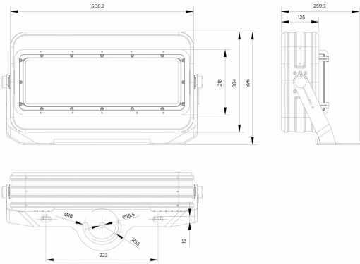
BVP581 LED832/757 600W A35NB R5BV
