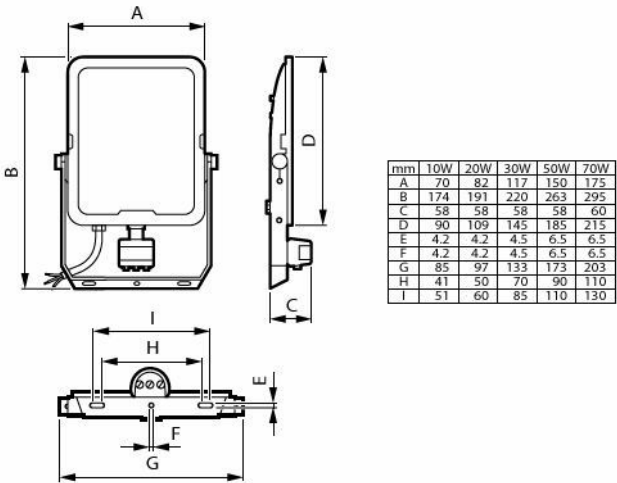
BVP167 LED60/830_40_65 PSU 50W SWB MDU
