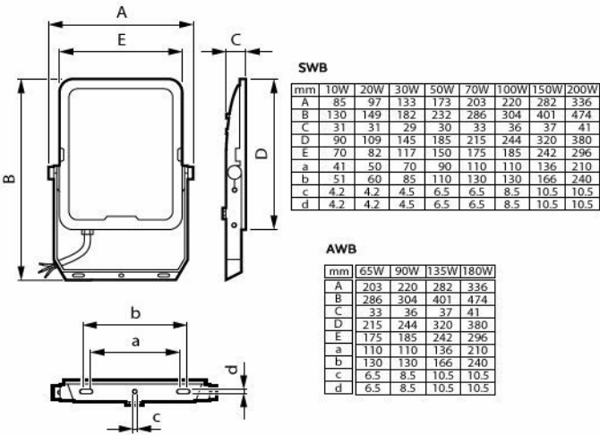
BVP169 LED240/830_40_65 PSU 200W SWB
