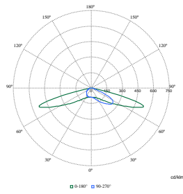
Polar Normal (separate) - BRP775I - 912300023483
