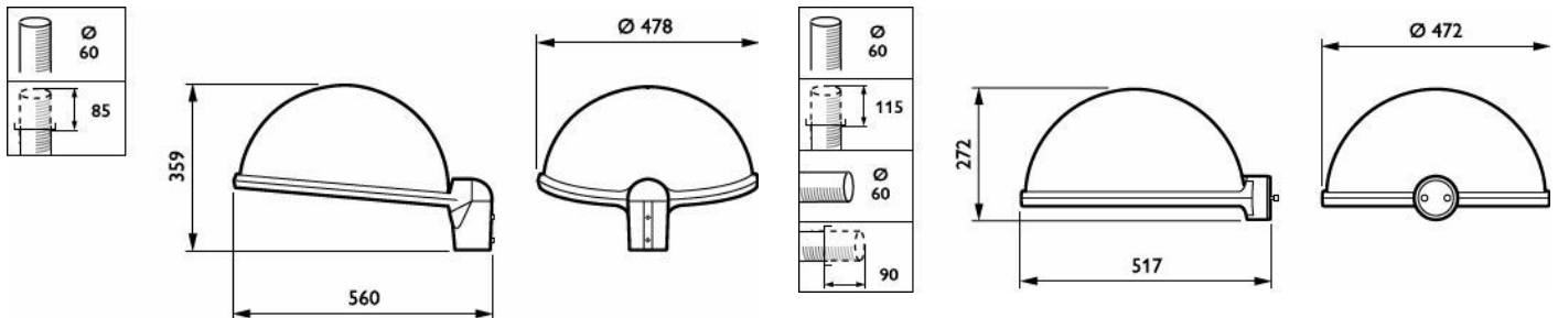
QUEBEC LED - LED module 4900 lm - 4th generation, screw fixation - 25 °C
