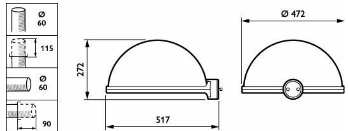
QUEBEC LED - LED module 4900 lm - 4th generation, screw fixation - 25 °C
