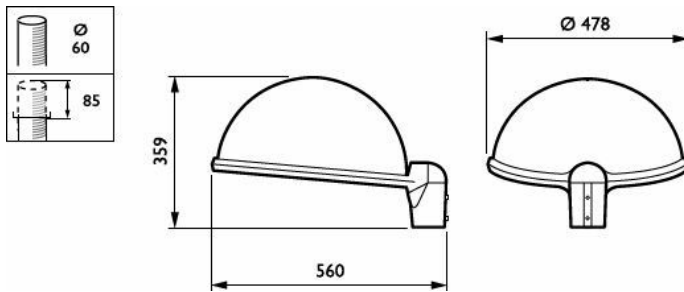
QUEBEC LED - LED module 4900 lm - 4th generation, screw fixation - 25 °C
