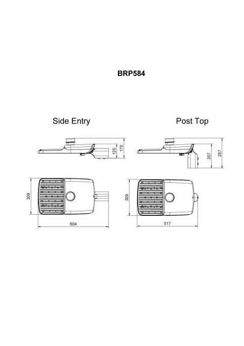
BRP584 LED379/NW 250W DM PSRD
