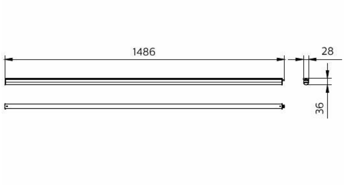
BN021C LED25S/840 L1500
