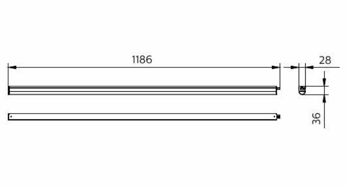
BN021C LED20S/840 L1200
