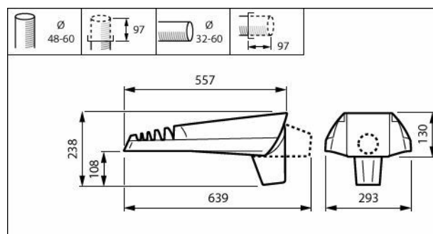
BGP702 LED40-4S/740 DM10 GF SRT SRB 60/7
