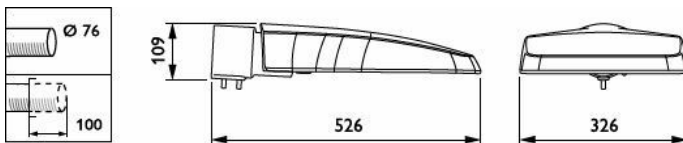
BGP307 LED120-4S/740 | DM11 48/76S
