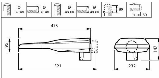
UniStreet gen2 Micro - dimensional drawing
