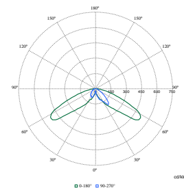
Polar Normal (separate) - BDP651 - 912300060159
