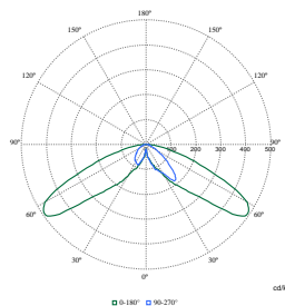
Polar Normal (separate) - BDP651 - 912300060157
