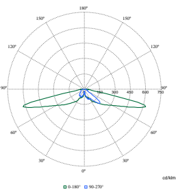
Polar Normal (separate) - BDP651 - 912300060274
