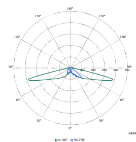
Polar Normal (separate) - BDP651 - 912300024529
