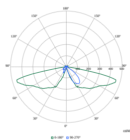
Polar Normal (separate) - BDP510I - 912300060140
