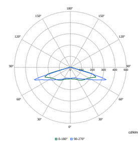
Polar Normal (separate) - BDP100I - 910500991087
