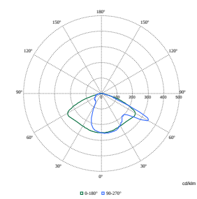
Polar Normal (separate) - BDP100I - 910925868115
