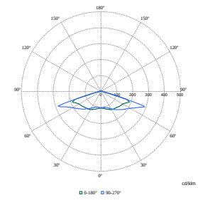
Polar Normal (separate) - BDP100I - 910925866282
