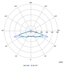
Polar Normal (separate) - BDP100I - 910500991210
