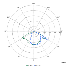
Polar Normal (separate) - BDP100I - 910925868067
