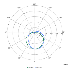
Polar Normal (separate) - BDP100I - 910925866290
