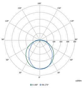
Polar Normal (separate) - BDP100I - 910500991095
