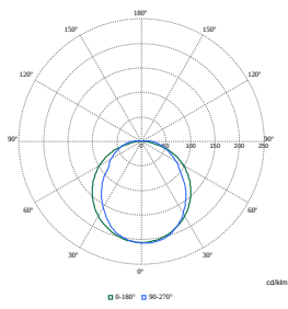
Polar Normal (separate) - BDP100I - 910500991102
