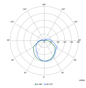
Polar Normal (separate) - BDP100I - 910925866281
