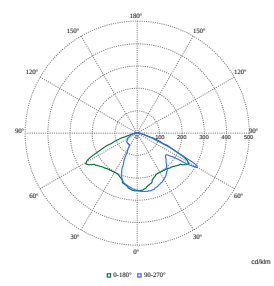
Polar Normal (separate) - BDP100I - 910925866624
