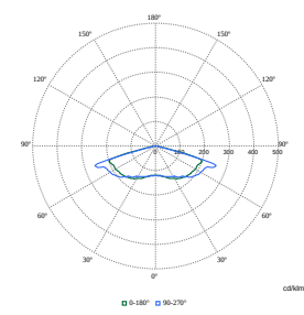
Polar Normal (separate) - BDP100I - 910925868116
