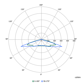
Polar Normal (separate) - BDP100I - 910500991098
