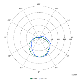
Polar Normal (separate) - BDP100I - 910925866279
