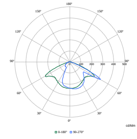
Polar Normal (separate) - BDP100I - 910925866278
