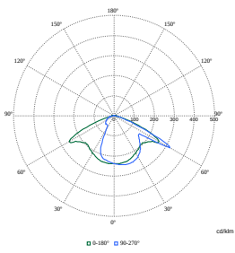
Polar Normal (separate) - BDP100I - 910500991070
