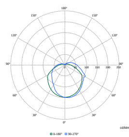
Polar Normal (separate) - BDP100I - 910925866292
