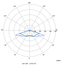
Polar Normal (separate) - BDP100I - 910925866295
