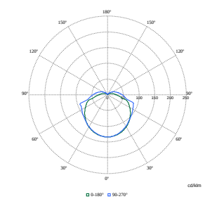
Polar Normal (separate) - BDP100I - 910500991190
