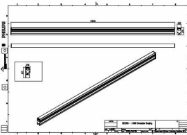
BCS340 48LED 40K 24V OC L100
