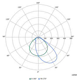
Polar Normal (separate) - BBP333I - 910925866266
