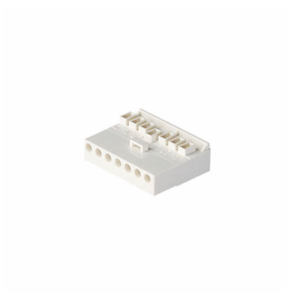
Electrical supply connector 7- pole
