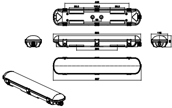
WT072C LED SW78CCT L600 PSU Wide
