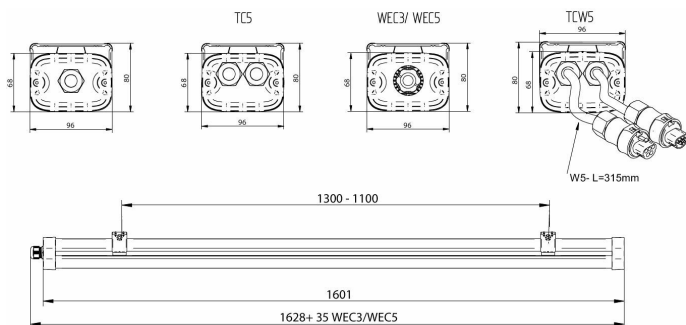
WT490C 645/840 PSD HE WB PI5 L1600
