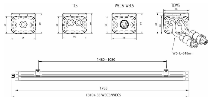
WT490C 100S/840 PSD HE WB PI5 L1800
