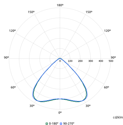
WT490CI - 910925868692
