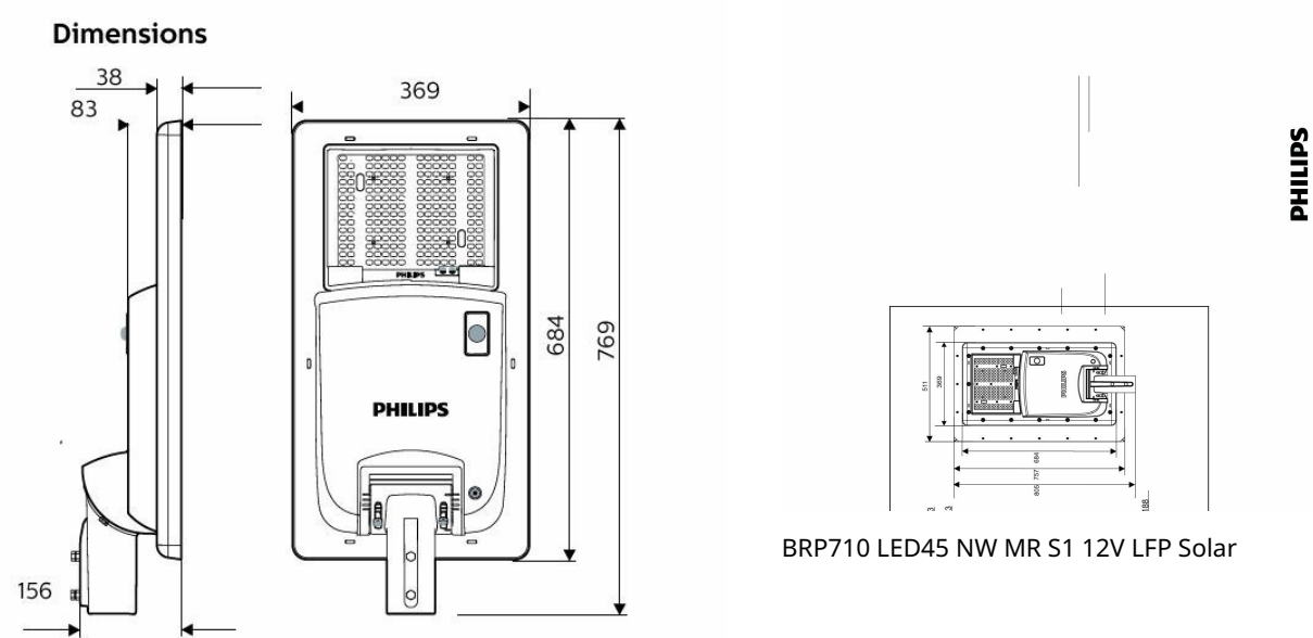
BRP710 LED30 NW MR 12V LFP AIO Solar
