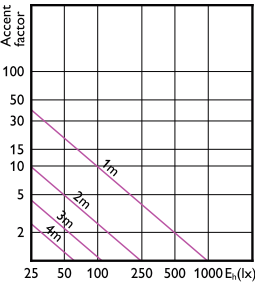
Accent Diagram - 5.5PAR20/COR/ F40/930/DIM/P/T20 6/1FB
