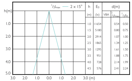
Beam diagram - Master LED PAR30L 32W 30D 857
